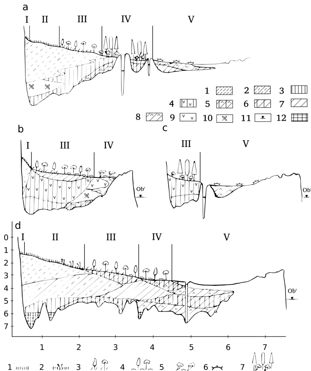
Figure 4. Stratigraphic structure of peat deposits of floodplain mires of the Ob' River valley in the south of the forest zone of Western Siberia (Subtaiga zone).
