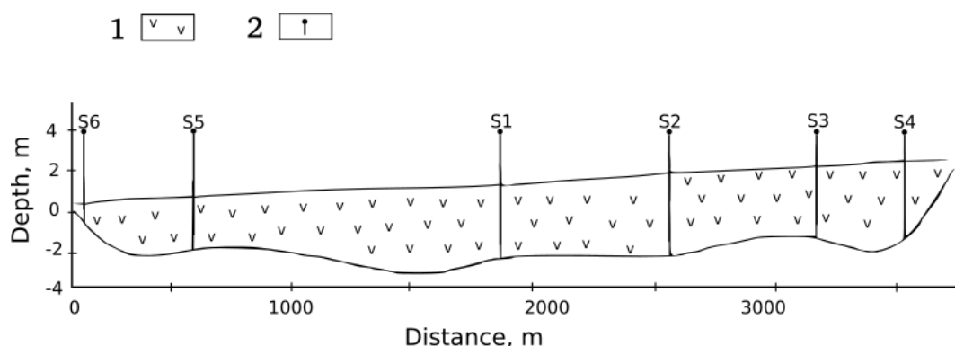
Figure 5. Profile of peat deposits of the Semenovskoe mire on the left-bank valley of the Iksha River ('Borodinsk' key area, Southern taiga subzone).
